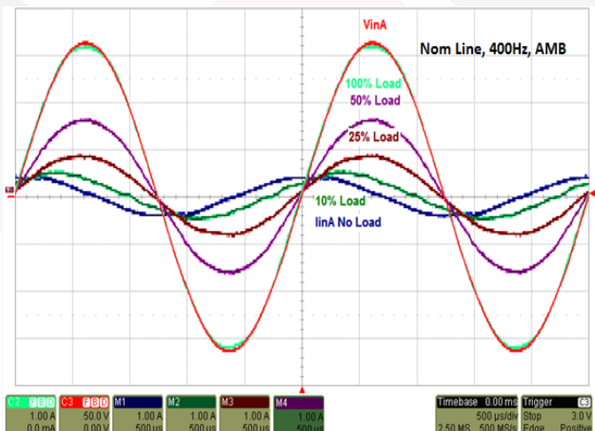
Figure 5: Typical 400 Hz input current waveforms (only Phase A shown); includes MACF-115-3PH-UNV-QG external input filter module.
