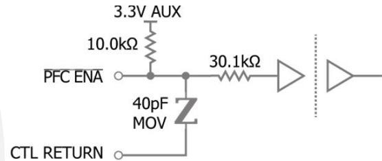
Figure 21: Internal circuitry for PFC ENA pin.
