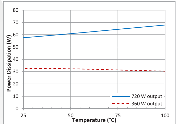
Figure 3: Power dissipation vs. baseplate temperature. Load applied at +VOUT. Input: 60 Hz 3-phase 115 Vrms (L-N).
