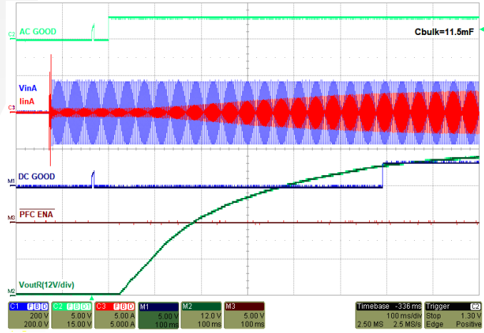
Figure 7: Full-Load (Resistive) startup into 11.5mF (for clarity, only Phase A of the input voltage and current are shown).
